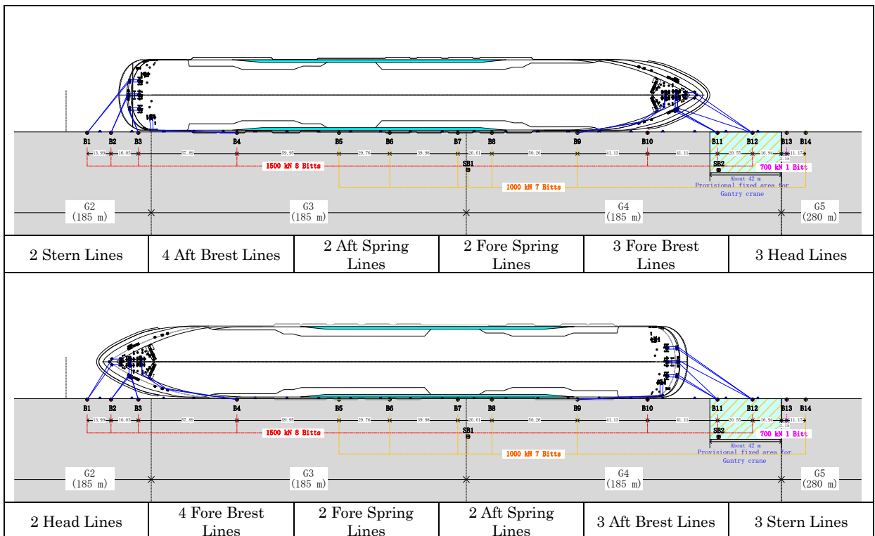
Figure 1.3.4 Recommended mooring position for passenger vessels of 160,000GT [FY 2017]
