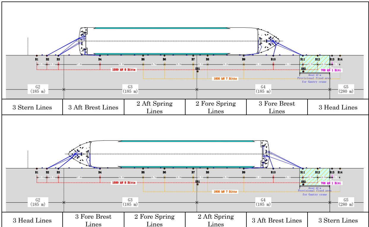
Figure 1.3.2 Recommended mooring position for passenger vessels of 110,000GT [FY 2017]
