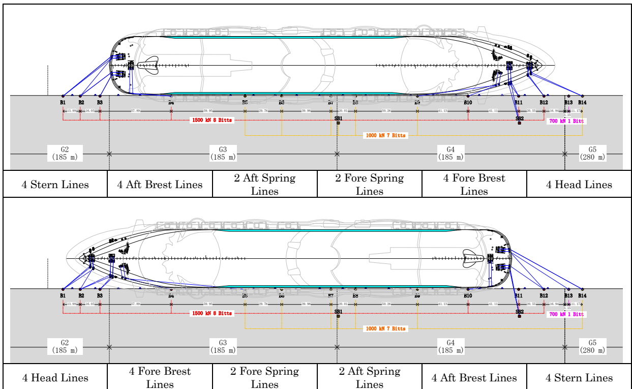
Figure 1.3.6 Recommended mooring position for passenger vessels of 220,000GT [FY 2018]
