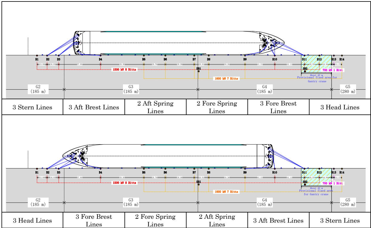
Figure 1.3.1 Recommended mooring position for passenger vessels of 80,000GT [FY 2017]
