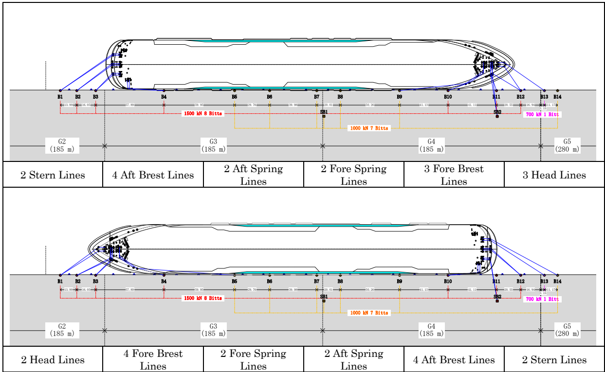
Figure 1.3.5 Recommended mooring position for passenger vessels of 160,000GT [FY 2018]
