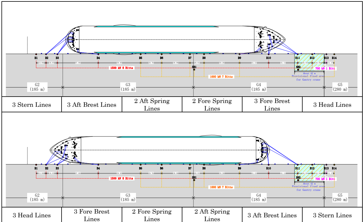
Figure 1.3.3 Recommended mooring position for passenger vessels of 130,000GT [FY 2017]
