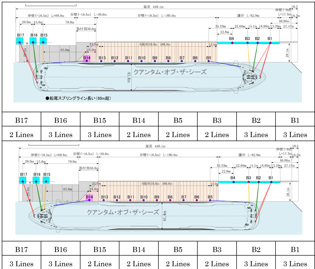
Figure 1.3.4 Recommended mooring position for passenger vessels of 160,000GT
